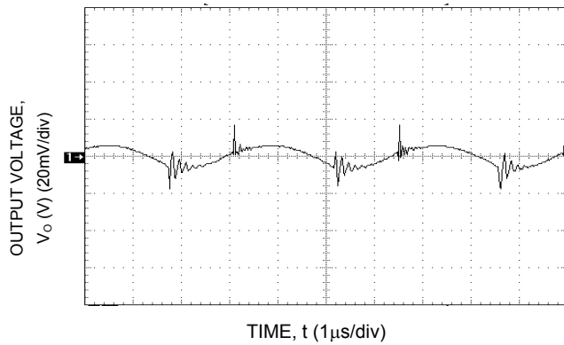
Figure 8. Typical Output Ripple and Noise.
