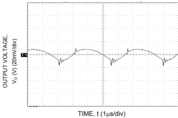
Figure 44. Typical Output Ripple and Noise.
