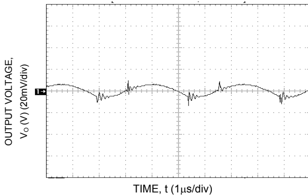
Figure 32. Typical Output Ripple and Noise.
