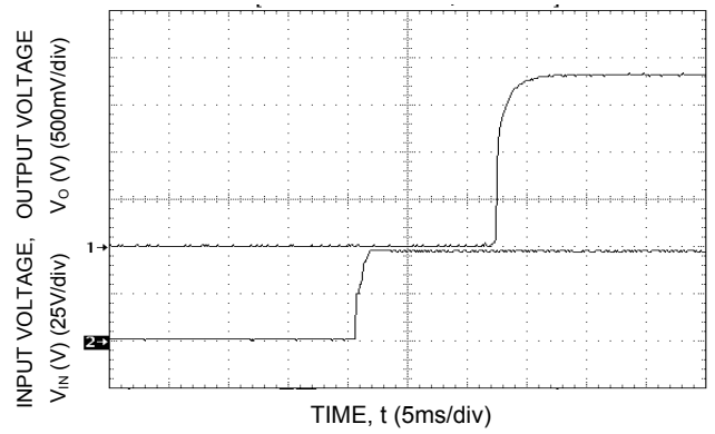
Figure 29. Typical Start-Up with application of Vin.
