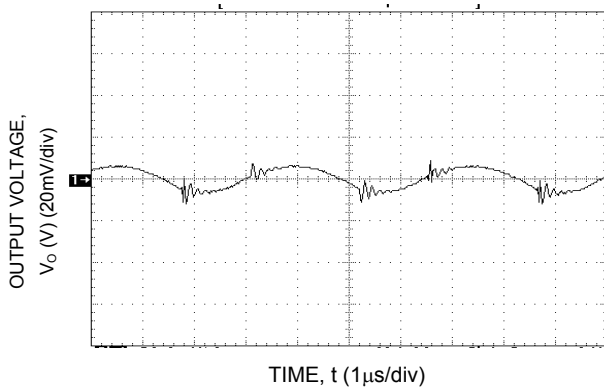
Figure 26. Typical Output Ripple and Noise.
