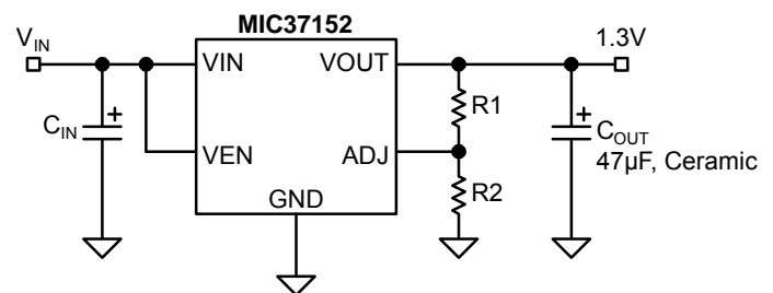
Adjustable Regulator
