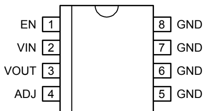
SOIC-8 (M)
