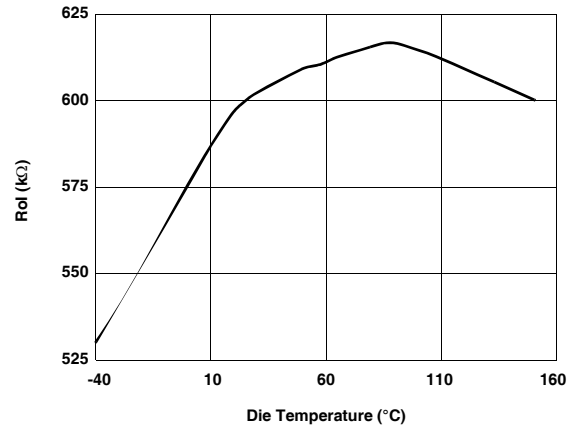
Transimpedance (RoI) vs Temperature
