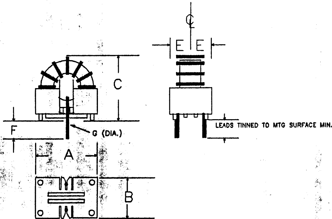
PC BOARD MOUNTING PATTERN
