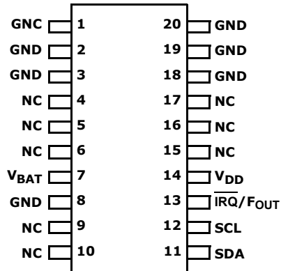
ISL12022MA (20 LD SOIC) TOP VIEW
