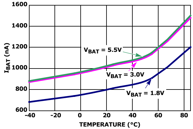
FIGURE 3. I_{BAT} vs TEMPERATURE ( V_{DD} = 0V )
