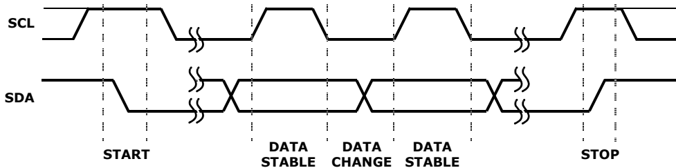
FIGURE 15. VALID DATA CHANGES, START AND STOP CONDITIONS
