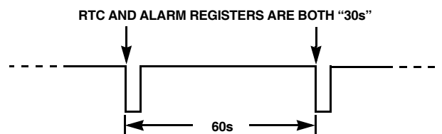
FIGURE 14. \overline{IRQ}/F_{OUT} WAVEFORM
