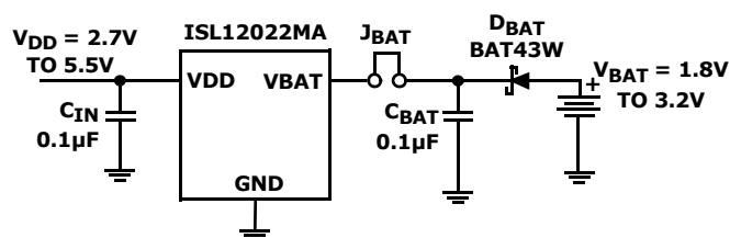
FIGURE 20. SUGGESTED BATTERY BACKUP CIRCUIT
