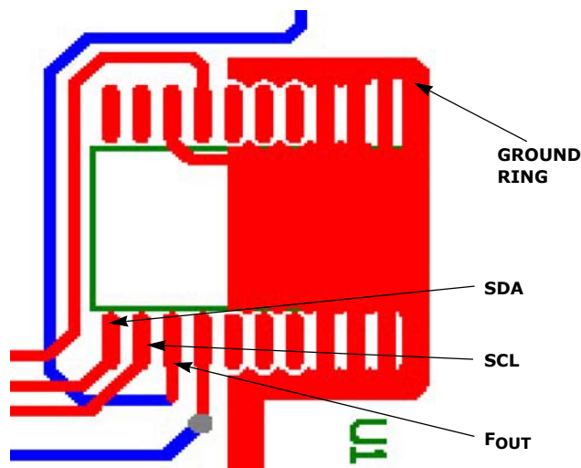
FIGURE 21. SUGGESTED LAYOUT FOR THE ISL12022MA
