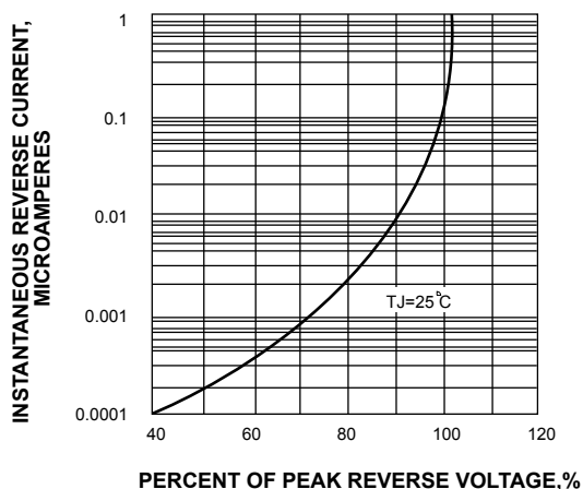
FIG. 2-REVERSE CURRENT VERSUS CONTINUOUS REVERSE VOLTAGE (TYPICAL VALUES)
