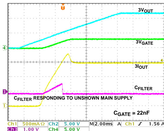
FIGURE 4. 3VMAIN START-UP R LOAD = 2Ω, C LOAD = 470μF
