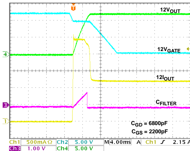
FIGURE 5. 12VMAIN START-UP R LOAD = 10Ω, C LOAD = 470μF
