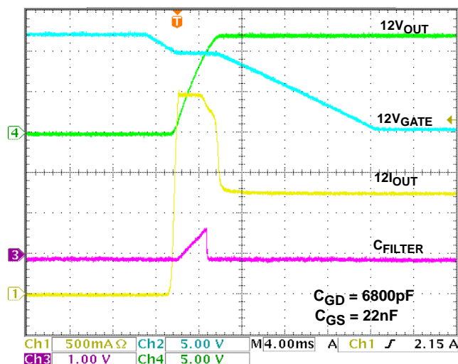
FIGURE 3. 12VMAIN START-UP R LOAD = 10Ω, C LOAD = 470μF
