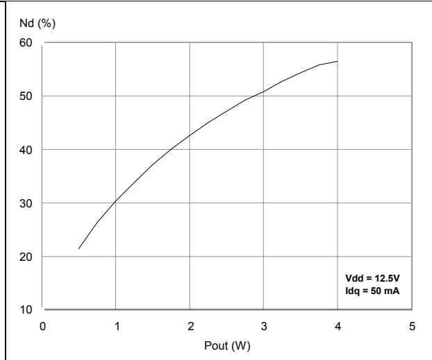
Figure 28. Drain efficiency vs output power
