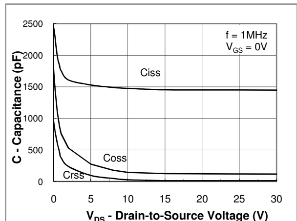
Fig.6 Capacitance
