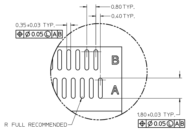
DETAIL Z SCALE 10:1
