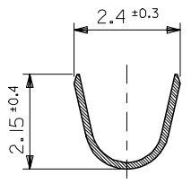
SECT B-B
