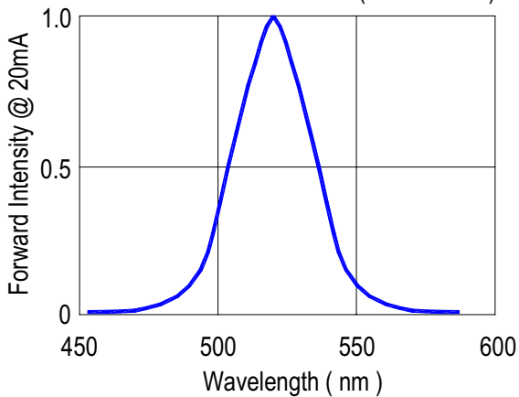
FIG. 5 Relative Intensity vs. Wavelength ( λp ) ( Ta = 25 °C )
