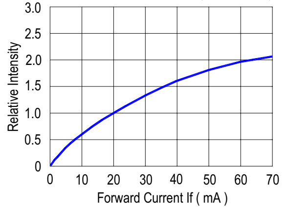
FIG. 2 Relative Intensity vs. Forward Current ( Ta = 25 °C )
