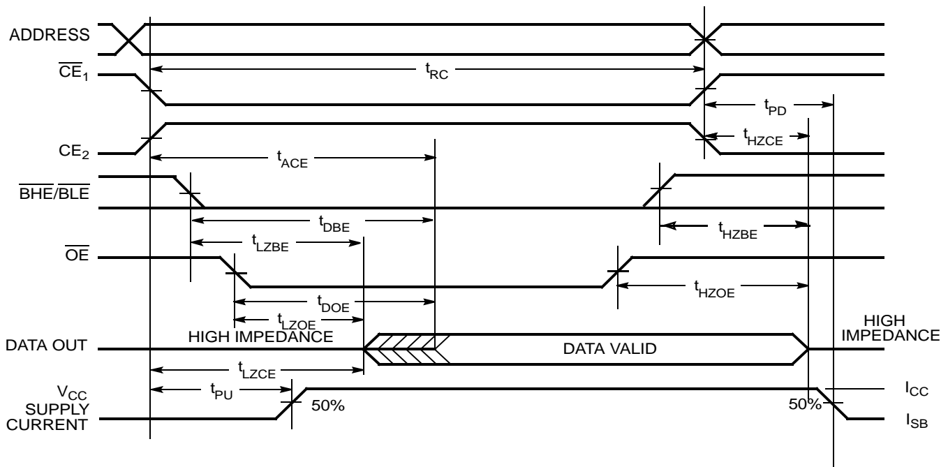
Figure 3. Read Cycle 2 ( \overline{\text{OE}} Controlled) [20, 21]
