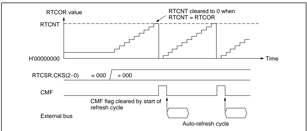
Figure 12.18 Auto-Refresh Operation
