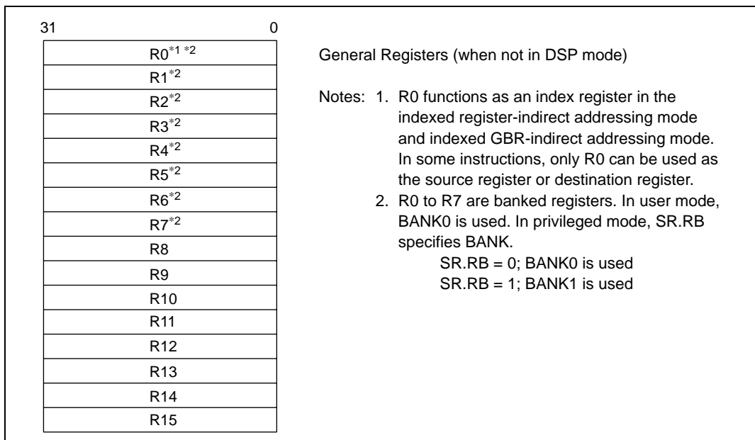
Figure 2.3 General Purpose Register (Not in DSP Mode)
