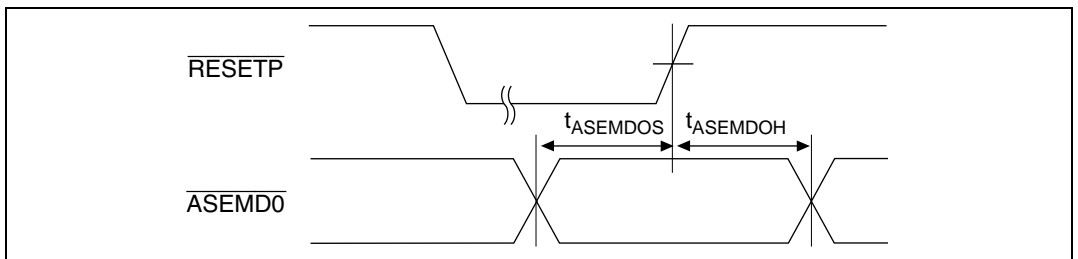
Figure 32.50 \overline{\text{ASEMDO}} Input Timing
