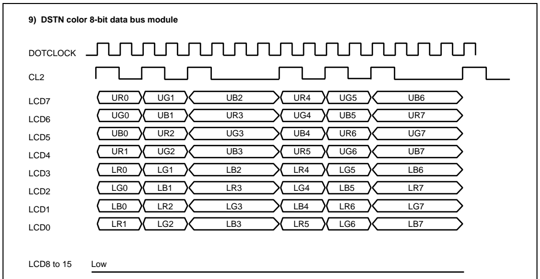
Figure 25.16 Clock and LCD Data Signal Example
