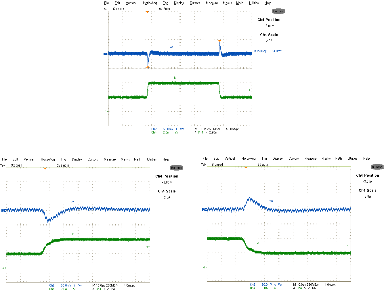
Fig. 23. Transient Response, 2A to 4A step 2.5A/μs Ch 2 :V o , Ch 4 :I o
