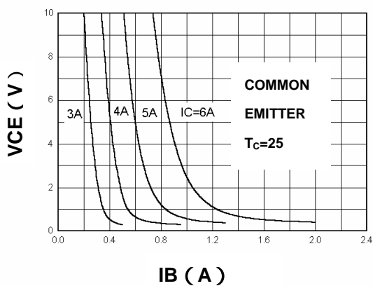
VCE - IB
