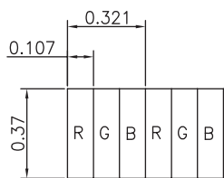
Detail A Scale 50:1
