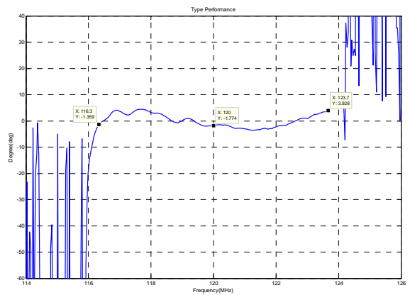
Phase Linearity(f0±3.4MHz)
