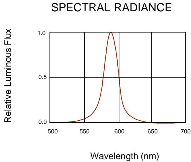
Fig.5 Relative Luminous Flux vs. Wavelength
