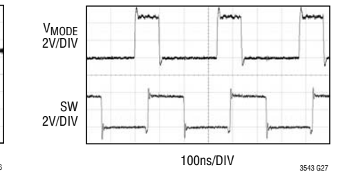
PLL Operation at 3MHz
