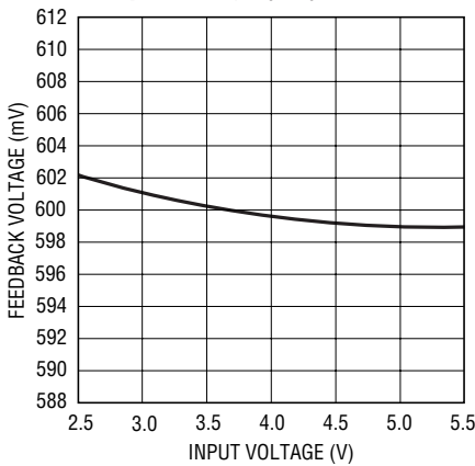
Feedback Voltage ( V_{FB} ) vs Input Voltage ( V_{IN} )
