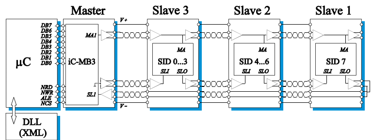
Figure 2: Example network of iC-MB3 and three subscribers. All 8 possible slave IDs (SIDs) are used distributed.
