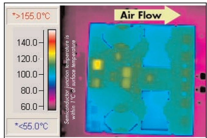
Figure 6: Thermal plot of converter at 23 amp load current with 55°C air flowing at the rate of 200 LFM. Air is flowing across the converter from input to output (nominal input voltage).
