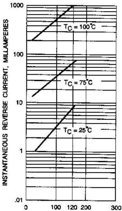
Fig. 3-TYPICAL REVERSE CHARACTERISTICS
