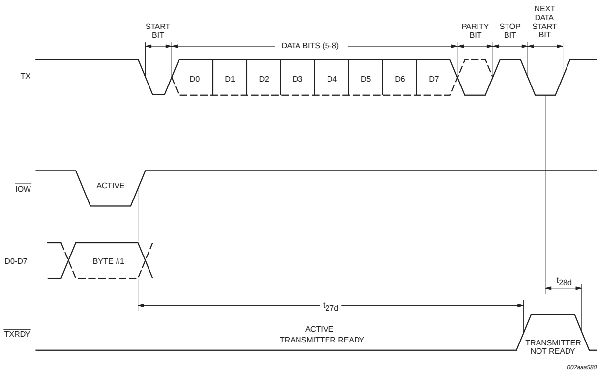
Fig 14. Transmit ready timing in non-FIFO mode.
