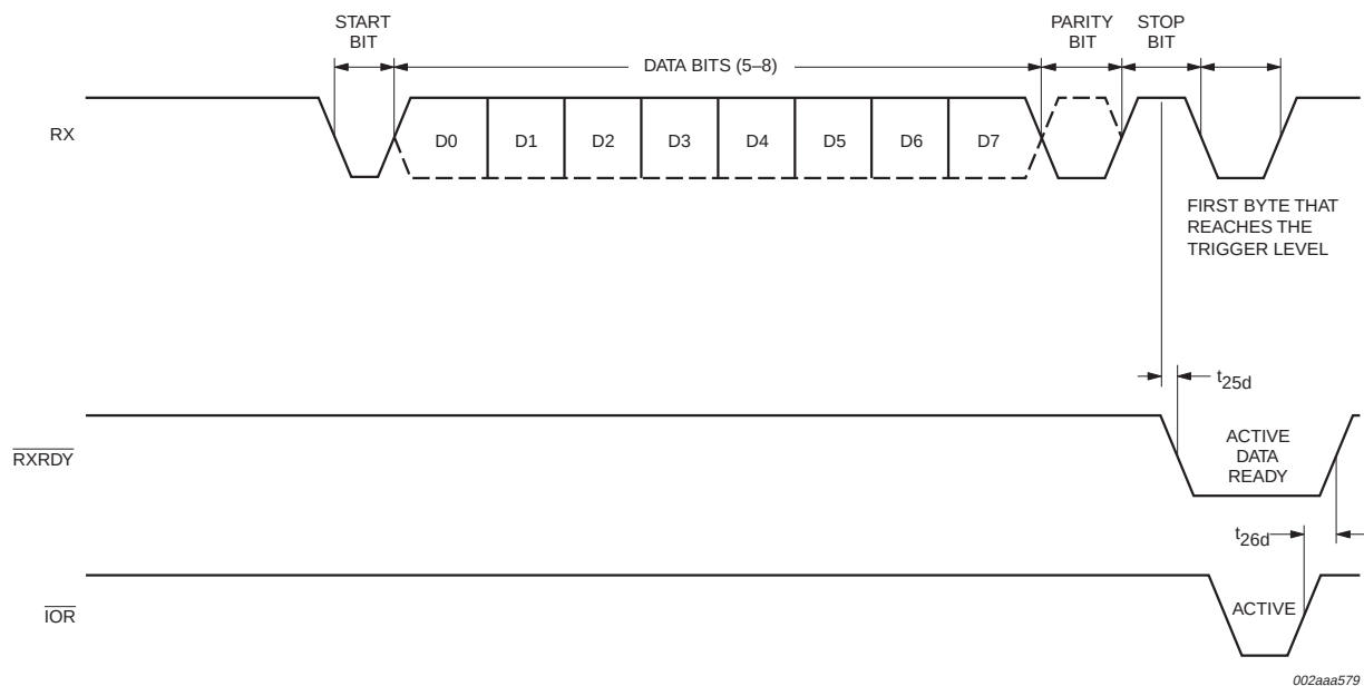
Fig 12. Receive ready timing in FIFO mode.
