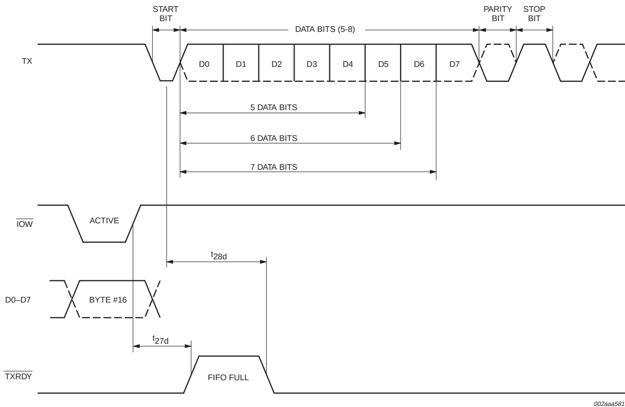
Fig 15. Transmit ready timing in FIFO mode (DMA mode '1').
