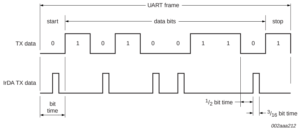
Fig 16. Infrared transmit timing.
