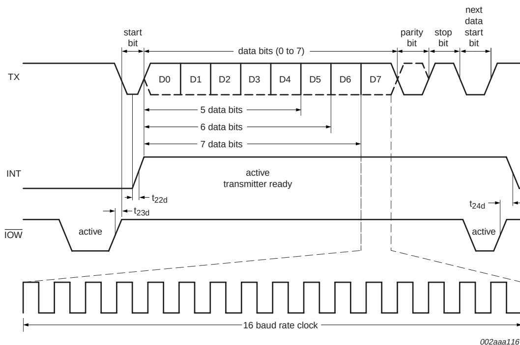
Fig 13. Transmit timing.
