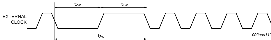
Fig 9. External clock timing.
