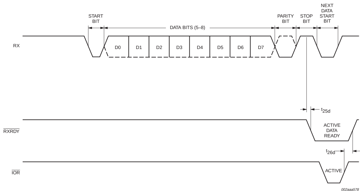
Fig 11. Receive ready timing in non-FIFO mode.
