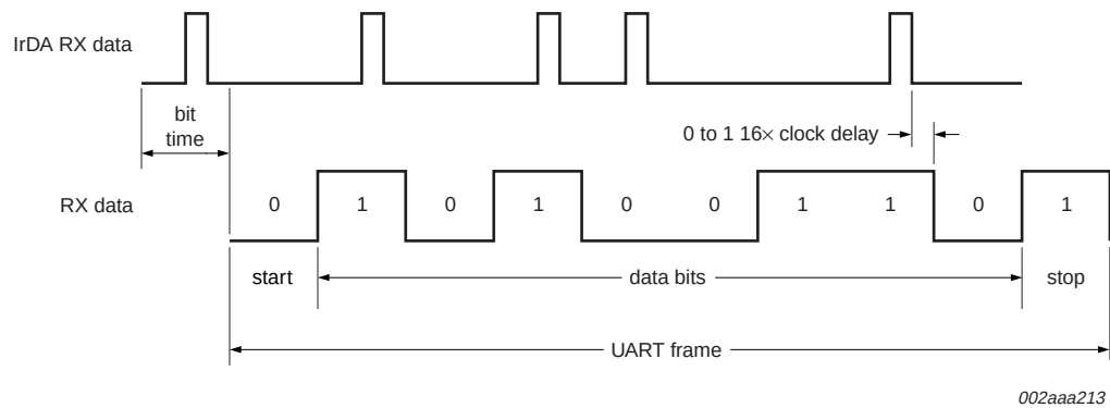
Fig 17. Infrared receive timing.
