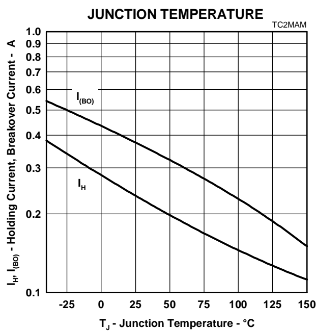
HOLDING CURRENT & BREAKOVER CURRENT VS JUNCTION TEMPERATURE
