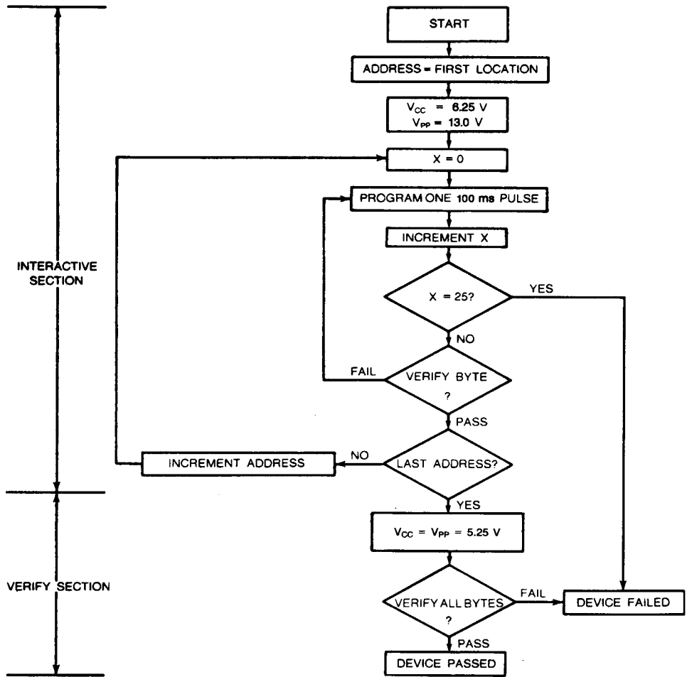
Figure 2. Flashrite Programming Flow Chart
