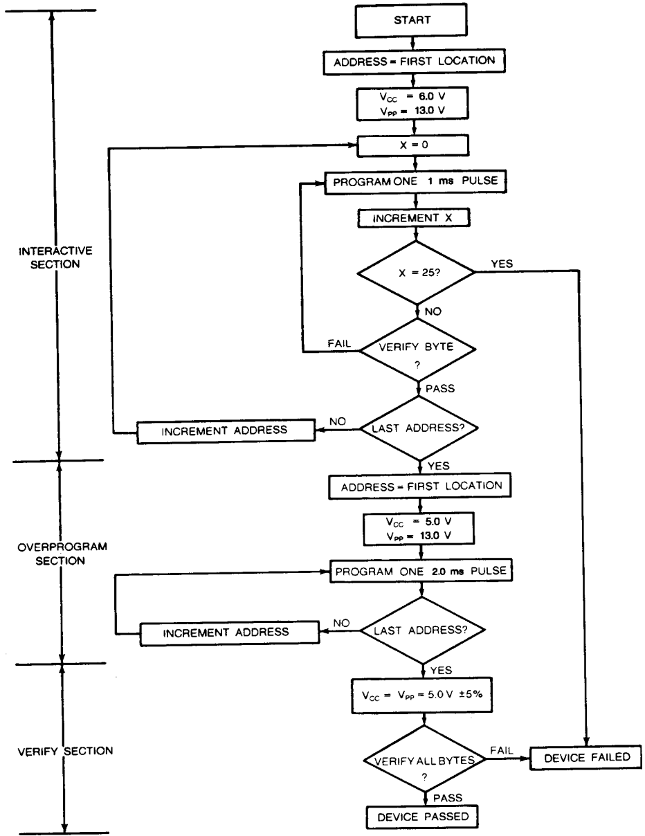
Figure 1. Interactive Programming Flow Chart
