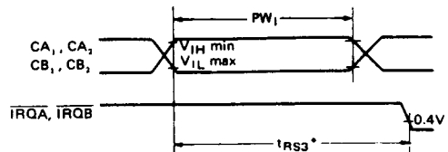
Figure 8 Interrupt Pulse Width and \overline{IRQ} Response
