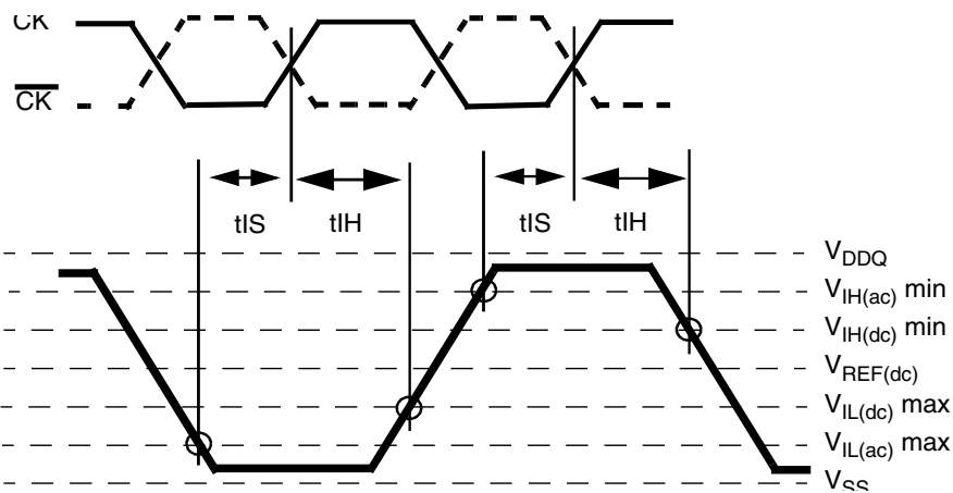
Differential input waveform timing - t_{IS} and t_{IH}
