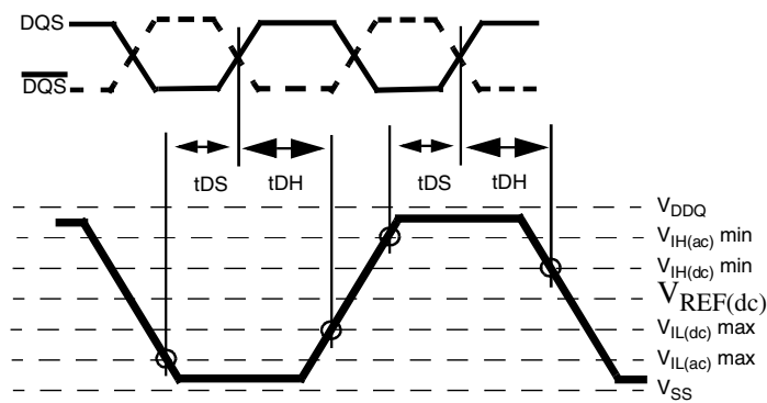
Differential input waveform timing - t_{DS} and t_{DH}
