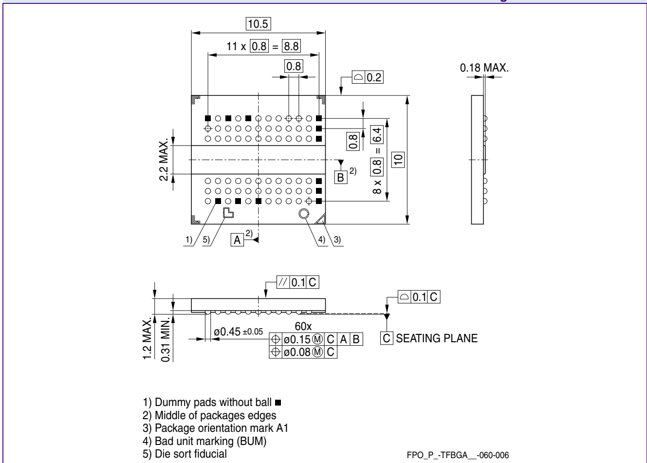
FIGURE 10 Package Outline P-TFBGA-60
