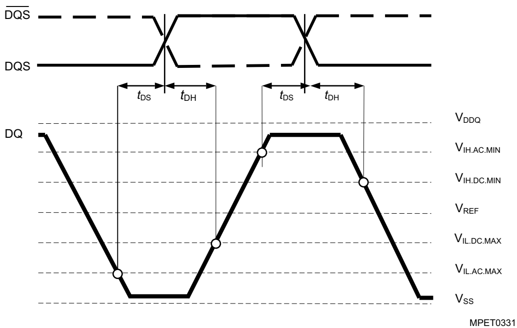
Differential Input Waveform Timing - t_{DS} and t_{DH}
