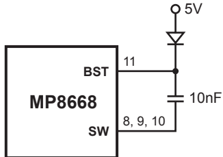
Figure 2—External Bootstrap Diode
