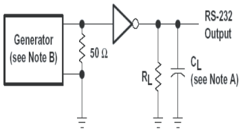
TEST CIRCUIT
