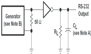
TEST CIRCUIT
