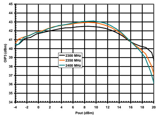
Figure 8. OIP3 vs. Pout and Frequency 2300 MHz – 2400 MHz
