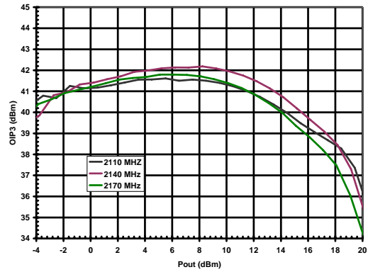
Figure 7. OIP3 vs. Pout and Frequency 2100 MHz – 2170 MHz
