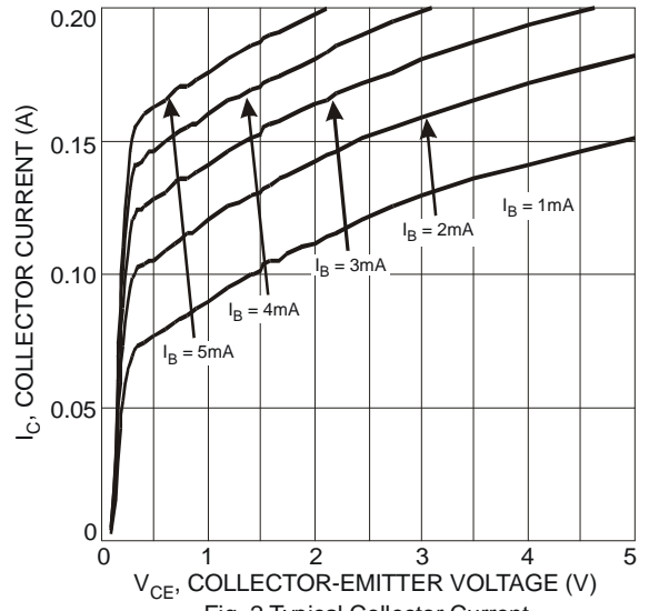
Fig. 2 Typical Collector Current vs. Collector-Emitter Voltage (DN0150BLP4)
