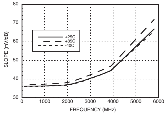
Slope vs. Frequency [1][2]
