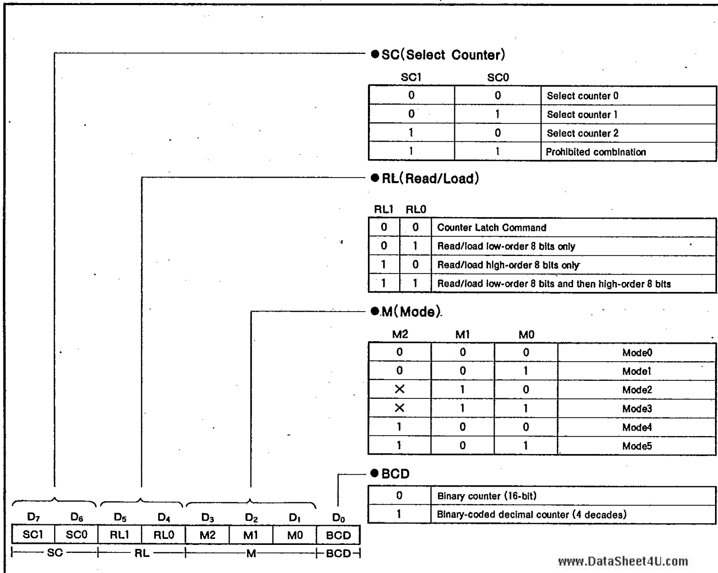
Fig. 1 Control-Word Format
