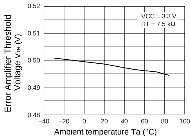
Error Amplifier Threshold Voltage vs. Ambient Temperature
