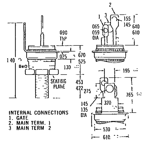
1/2" ISOLATED STUD MOUNT
