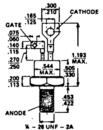
TO-48D
