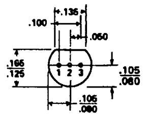
TO-92
