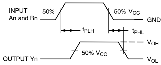
Figure 3. Switching Waveform
