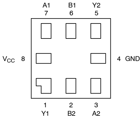
Figure 1. Pinout
