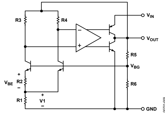
Figure 9. Simplified Schematic
