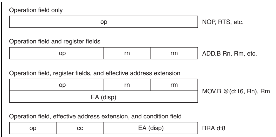
Figure 2.9 Instruction Formats
