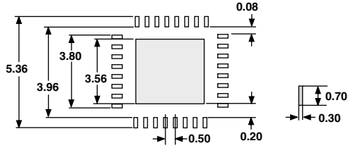
Figure 11. 5 mm × 5 mm LFCSP Pad Pattern
