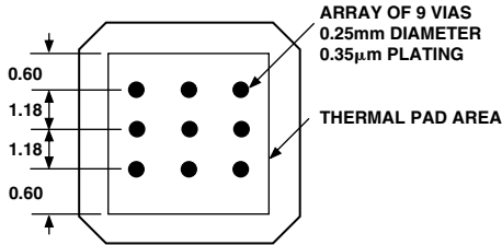
Figure 11. 5 mm × 5 mm LFCSP Pad Pattern
