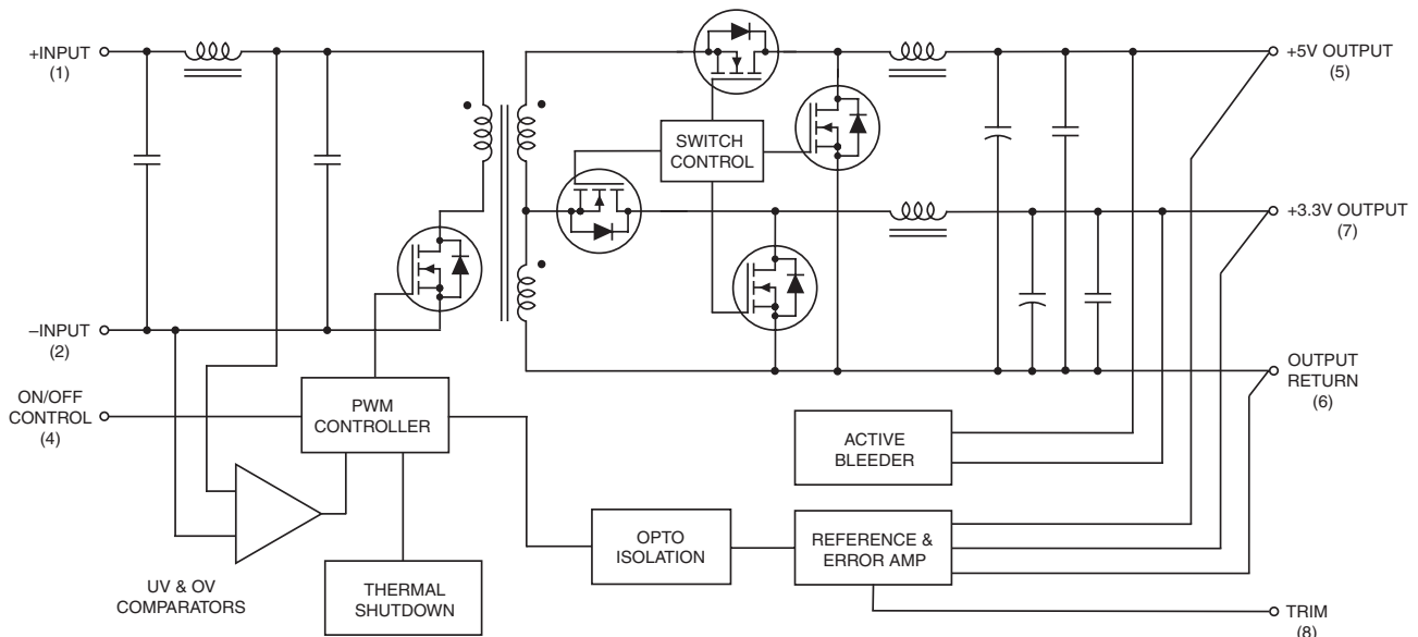
Figure 1. Simplified Schematic
