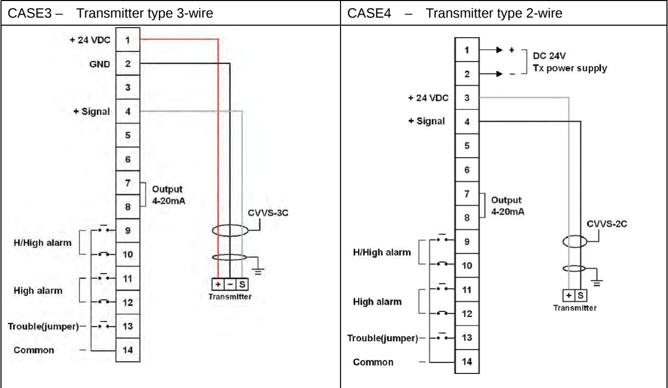
Fig. 6.2 The wiring method of GM-1000 single case and the wiring diagram.
