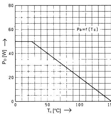
Allowable Power Dissipation vs. Tch
