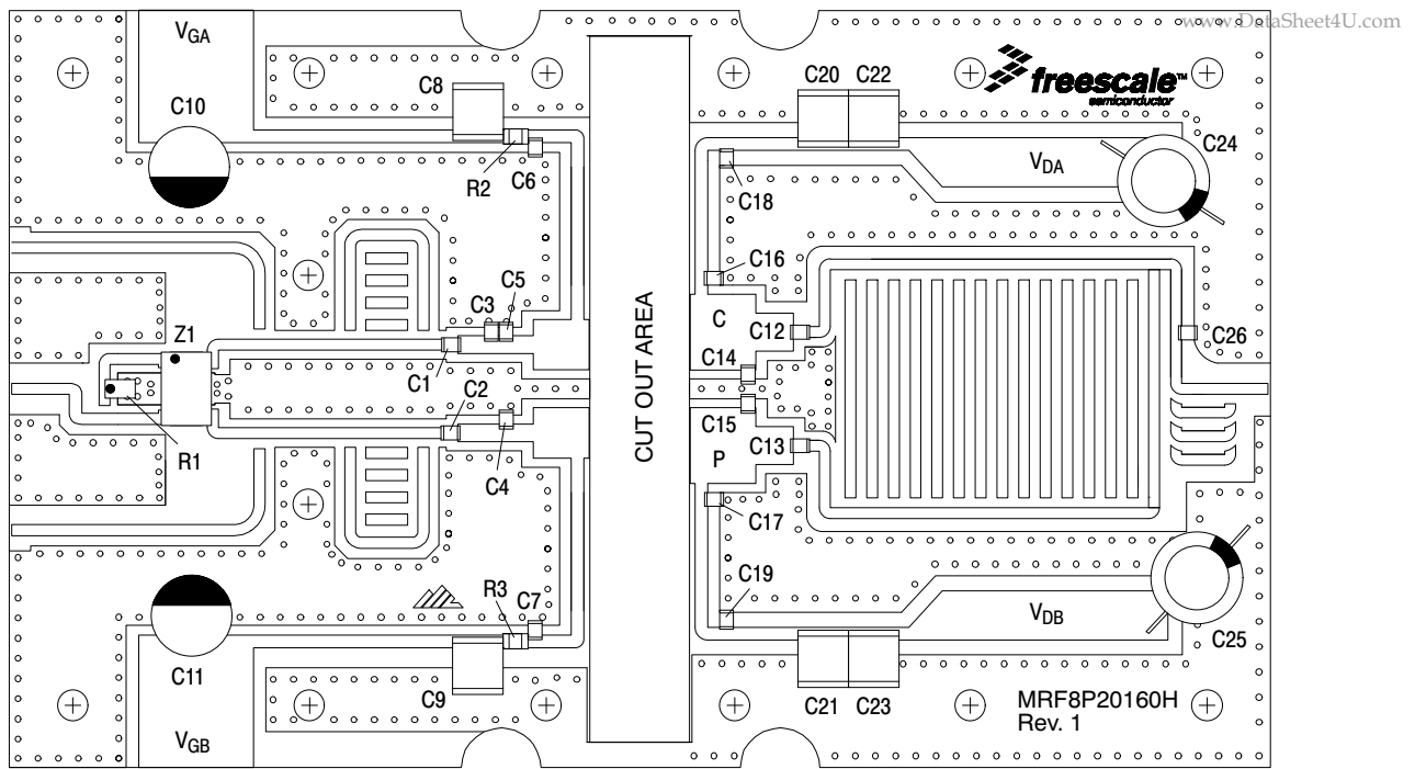
Figure 2. MRF8P20160HSR3 Test Circuit Component Layout
