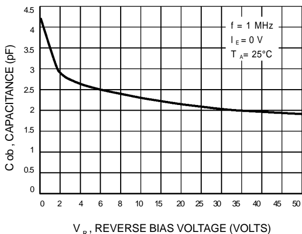
Figure 19. Output Capacitance
