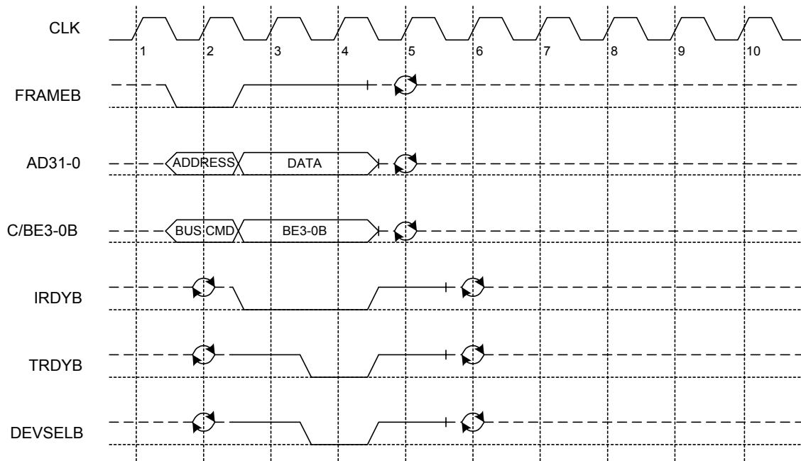
Figure 18. I/O Write
