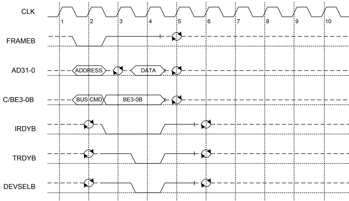
Figure 17. I/O Read
