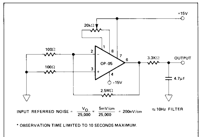
TYPICAL LOW-FREQUENCY NOISE TEST CIRCUIT*
