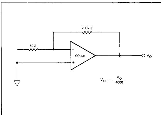
TYPICAL OFFSET VOLTAGE TEST CIRCUIT
