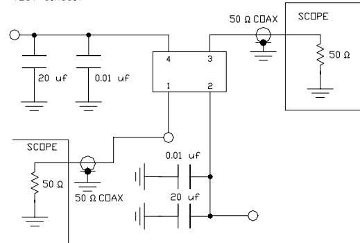
TEST CIRCUIT
